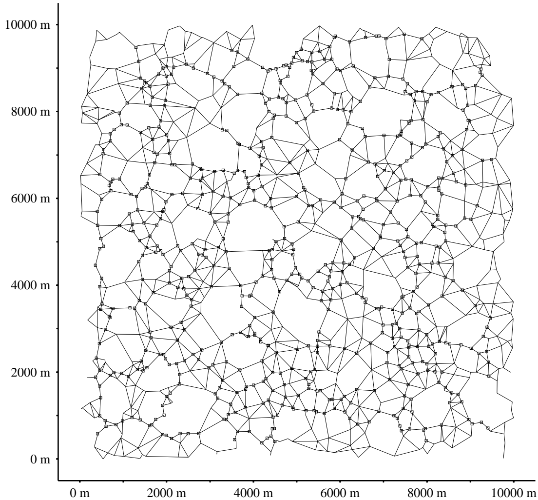
Figure 5.3: Stations with more than 1% of the end-to-end paths routed through them.
