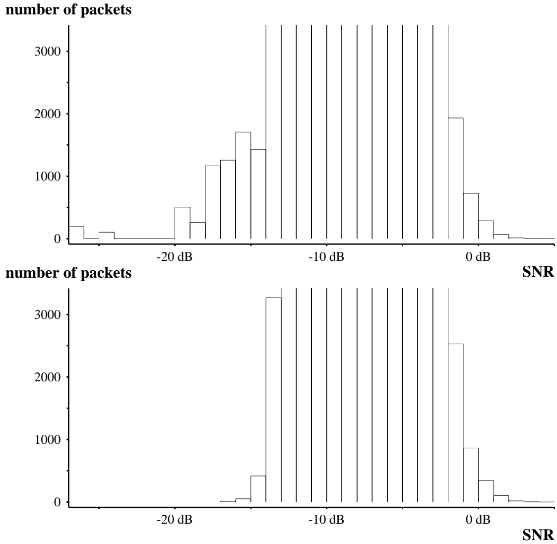
Figure 4.8: Same as Figure 4.7 but at a magnified vertical scale so that the tails can be seen more clearly. In the bottom distribution (for the case with the respect-neighbor constraint) no packets were received with a signal-to-noise ratio of less than -17 dB.
