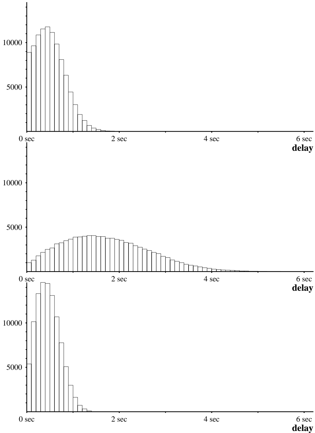
Figure 5.8: Distributions of measured end-to-end delays under extremely light load in simulated network. The top is for the network of 100 stations, the middle and bottom are for 1,000 stations. Both of these simulations used a slot size of \frac{1}{64} seconds with packet sizes of \frac{1}{1024} seconds. In the bottom plot the slot size was reduced to \frac{1}{256} seconds, reducing the average wait for a suitable scheduling slot by a factor of four.
