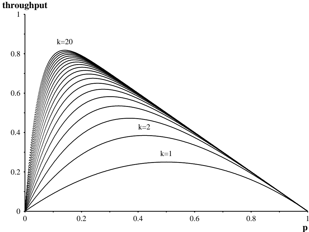
Figure 3.3: Variation of throughput, (1 - p) - (1 - p)^{k+1} , with receive duty cycle, p , for the number of neighbors k ranging from 1 to 20. Note that p near 0.3 produces good throughput for a wide range of k .
