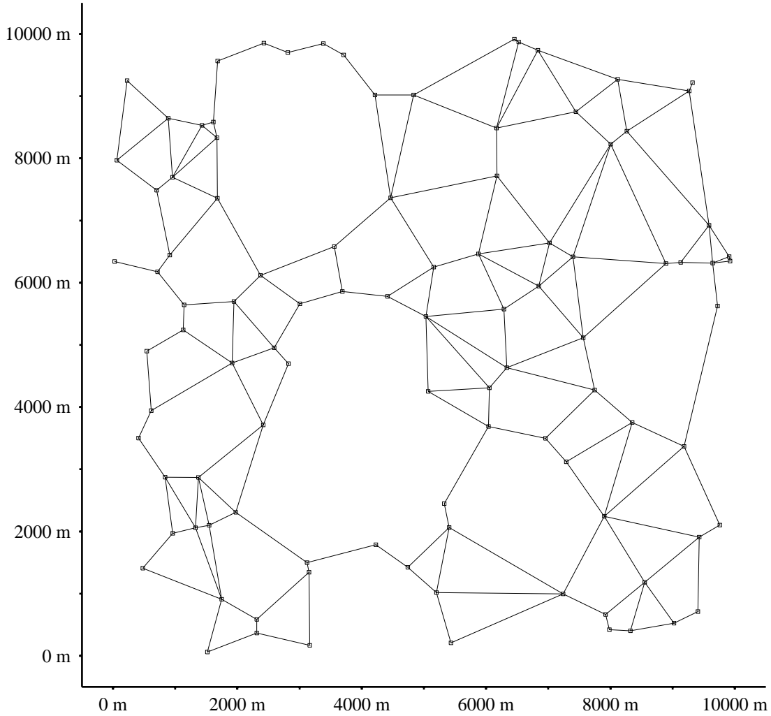
Figure 4.2: Direct hops used by minimum-energy routes.
