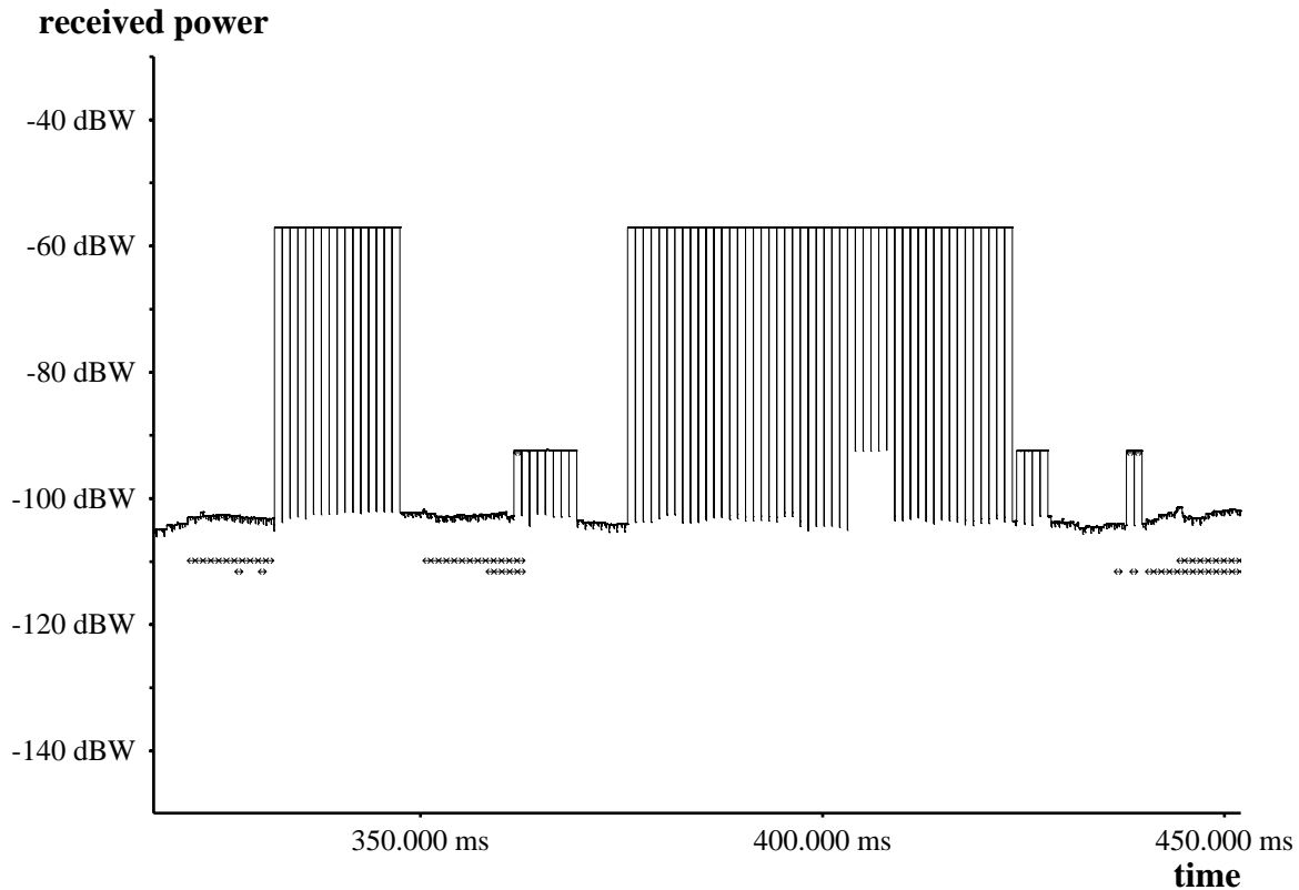
Figure 4.4: Simulation of received power at station number 29, with power control disabled. All transmissions are at -17 dBW, or 0.02 Watts, output power. As before, the lines with tiny arrowheads plotted below the received power level represent the receptions at this station and are plotted at the time and power level at which they are received. The variation in received power is a direct result of disabling the power control as it now depends on the distance (or path gain) between the stations. (Both the background noise level and the level of individual receptions are around 10 dB higher here than with power control, but that is the result of the particular fixed power level chosen for the transmissions. This 10 dB shift is not important. What is important is the signal-to-noise ratios, some of which are improved by use of power control, but the effect is too subtle to be seen by comparing this figure with the previous figure. We will be able to see the difference in Figure 4.5.)
