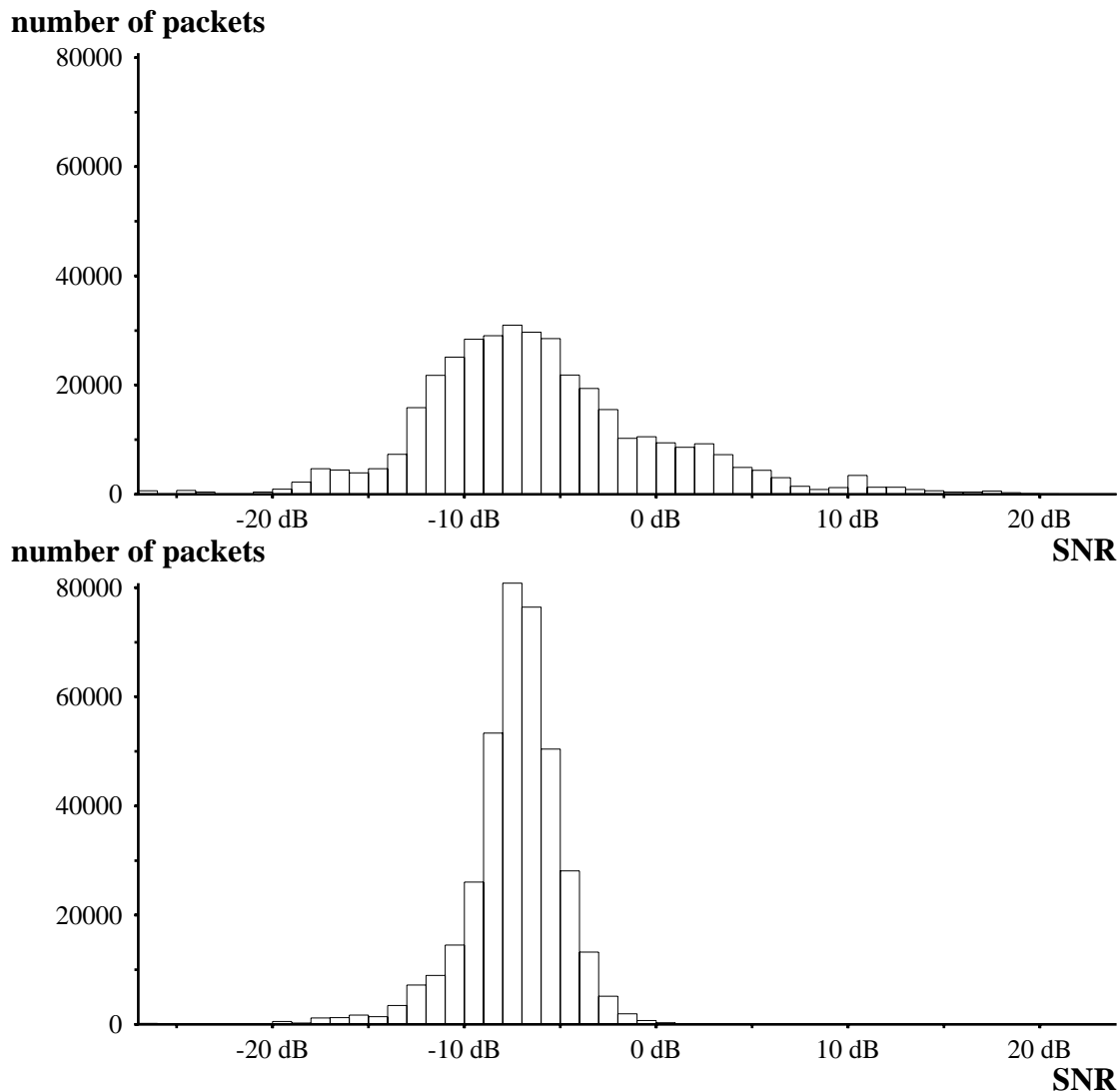
Figure 4.5: Distribution of worst signal-to-noise ratio during reception of each packet. Top plot is without power control and bottom plot is with power control.
