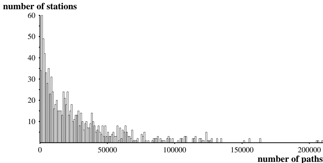
Figure 5.1: Distribution of number of paths routed through each station in the network of 1,000 stations using minimum energy routes (as shown in Figure 4.9). For each source-destination pair there is one path, for a total of 1,000,000 paths.
