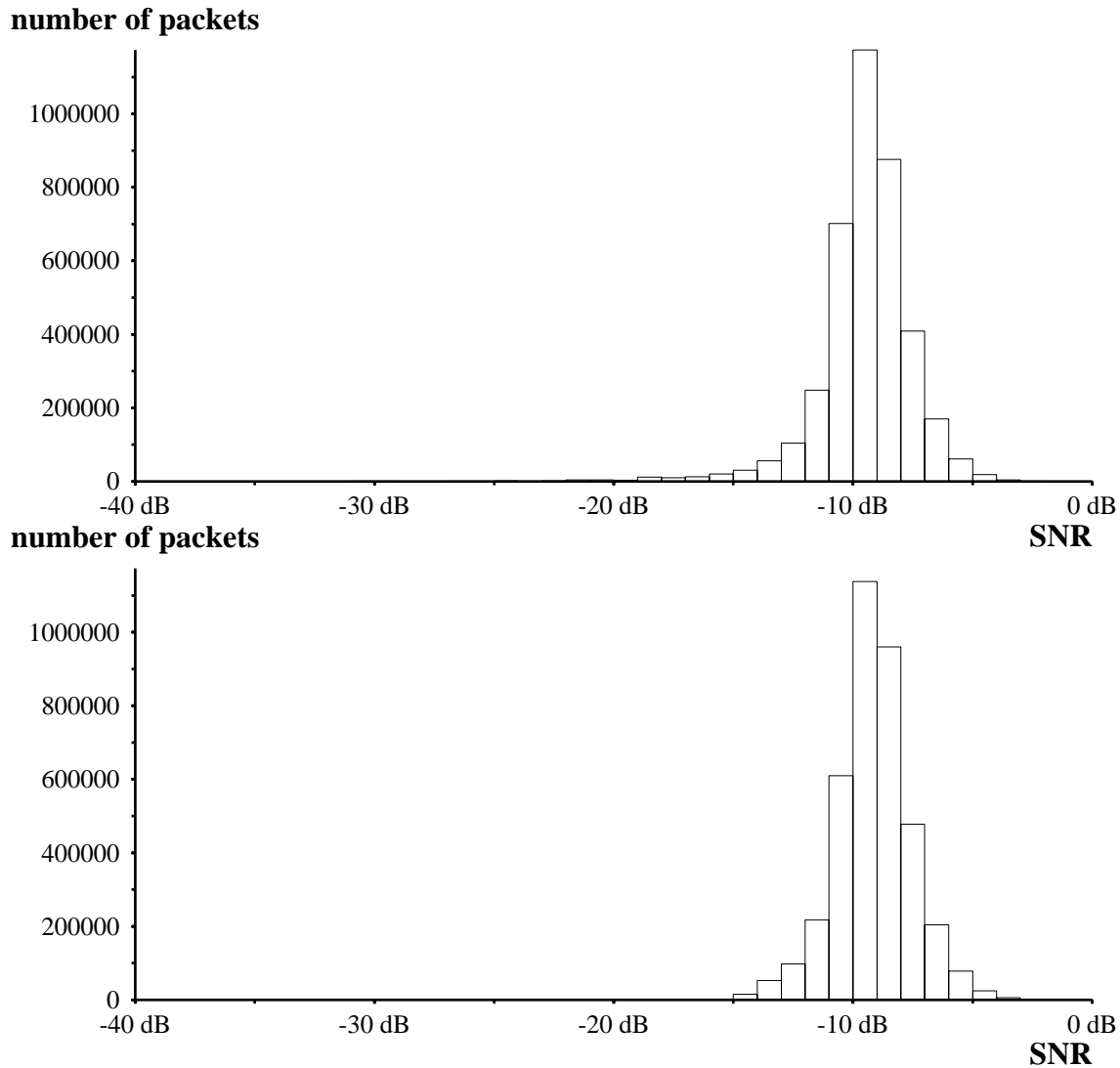
Figure 4.10: Signal-to-noise ratios for a network of 1,000 stations. The top plot is without, and bottom plot is with, the respect-neighbor constraint.
