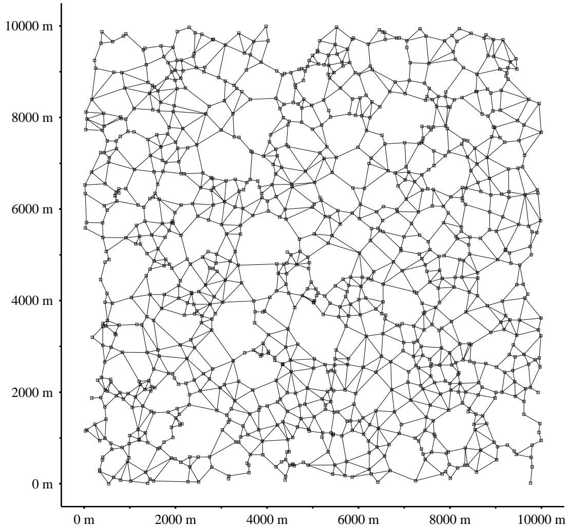
Figure 4.9: A network of 1,000 stations. Links shown are the direct hops used by minimum-energy routes.
