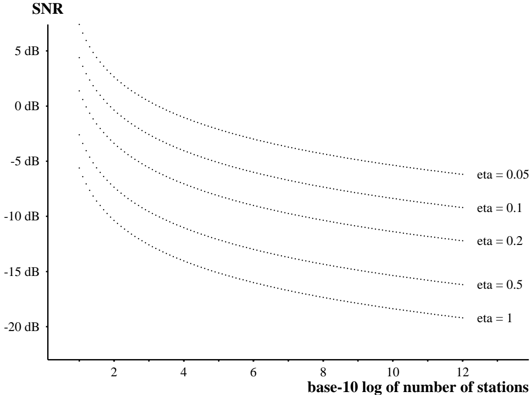
Figure 2.1: Decline of the signal-to-noise ratios as M , the number of stations, grows (Eq. 2.12). Each member of the family of curves is for a different value of the duty cycle, \eta .
