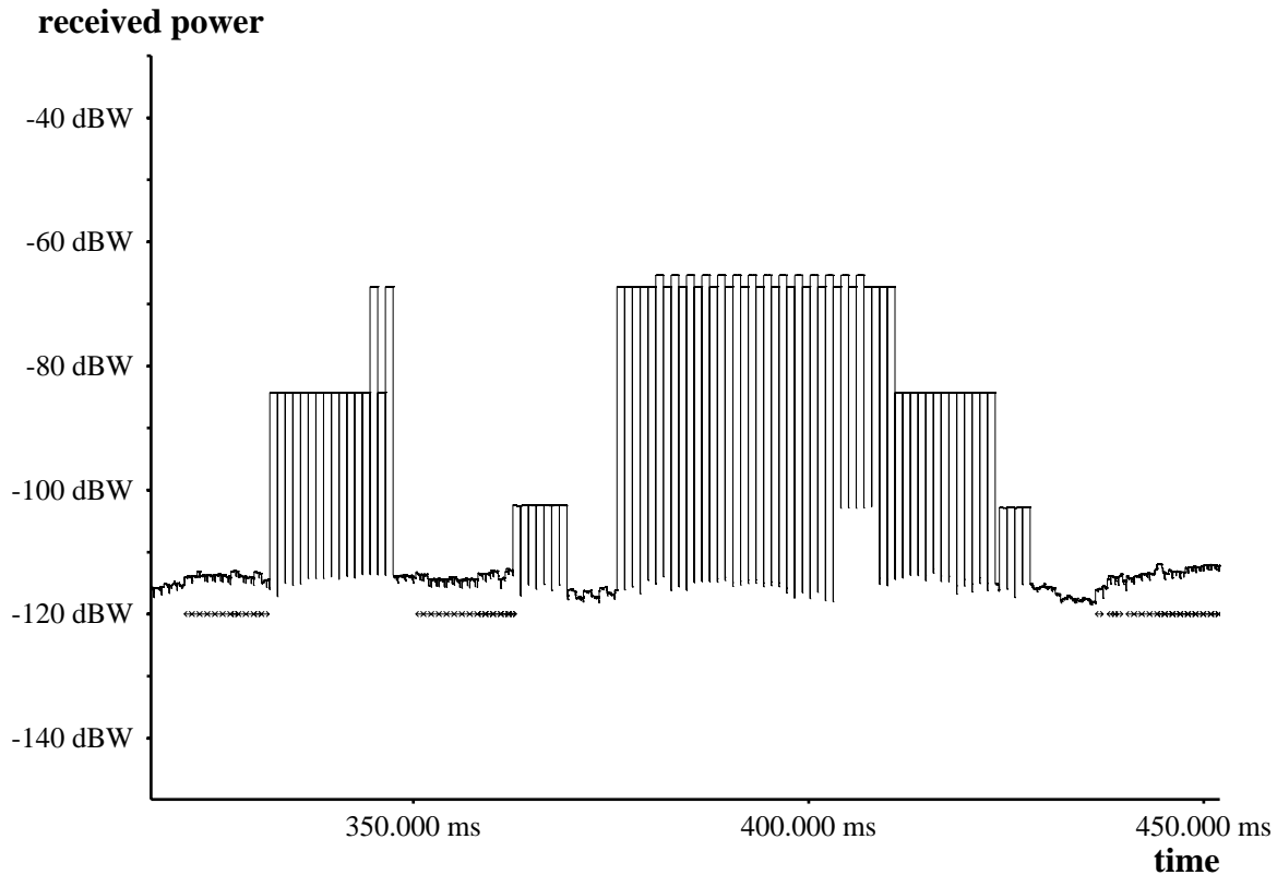
Figure 4.3: Example of received power as a function of time at station number 29 in the 100-station network. The lines with tiny arrowheads below the plotted receive power level are the receptions plotted at the time and power level at which they occur. Since power control is being used, all receptions occur at the same power level, -120 dBW. The higher levels of received power are caused by operation of the station’s own transmitter. The variation in the transmitter’s power level can be seen. (The receiver sees the transmitted power level down 40 dB.) A few of the high received power levels (those near -100 dBW) are caused by a transmitter at a nearby station (number 46 on the map in Figure 4.1).
