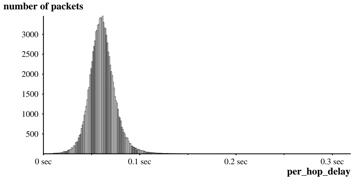
Figure 5.9: Distribution of measured end-to-end delays divided by number of hops, or the average per-hop delay, experienced by each packet in a lightly-loaded 1,000-station network with minimum energy routes, 64 slots per second, and 16 subslots per slot.
