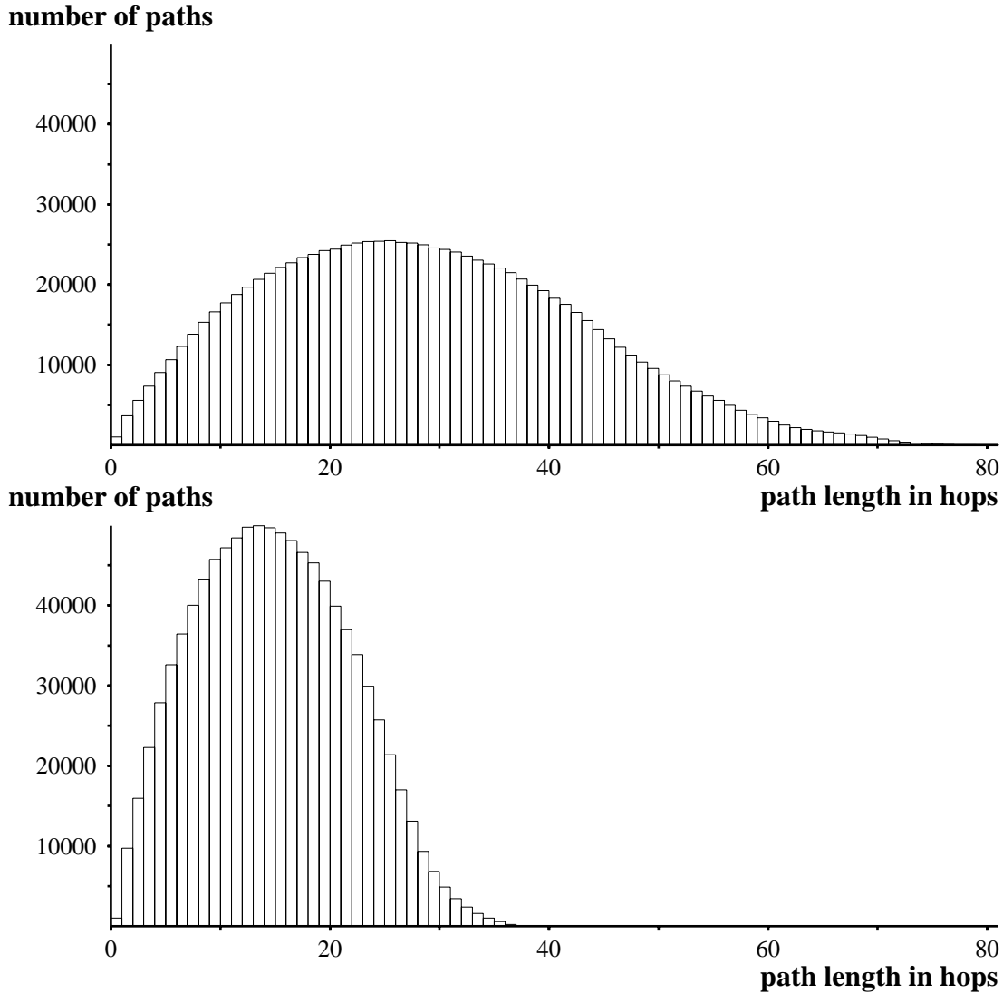
Figure 5.5: Distribution of path lengths of the 1,000,000 different paths in the network of 1,000 stations. The top plot is for minimum energy routes. The bottom plot is for the paths produced by the modified routing computation.
