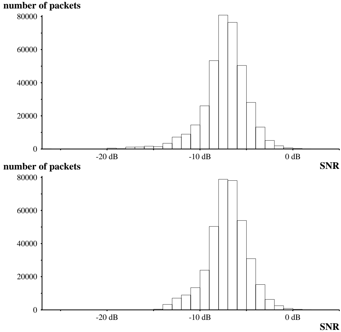
Figure 4.7: Impact of the respect-neighbor constraint on signal-to-noise ratio. Top distribution is the same as the bottom of Figure 4.5 (though the scale has changed) which is from a simulation with power control but without the respect-neighbor constraint. The bottom is with power control and with the respect-neighbor constraint. The respect-neighbor constraint has reduced to zero the number of packets received with low signal-to-noise ratio (this reduction can be seen more clearly in Figure 4.8 where the vertical scale is magnified), but has otherwise had little impact.
