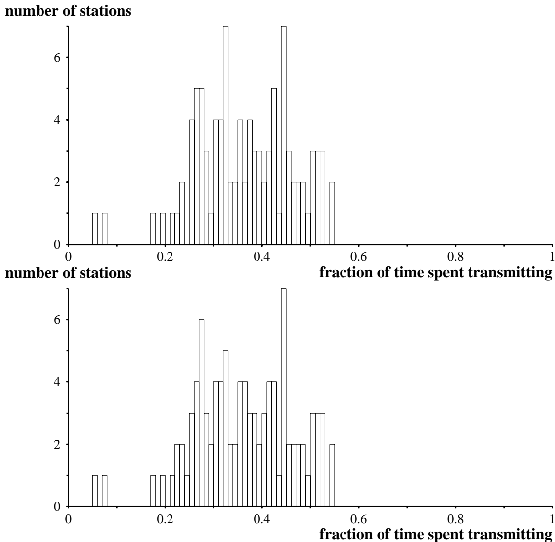
Figure 4.6: Distributions of the transmit duty cycle. The top is without the respect-neighbor constraint, and the bottom is with the respect-neighbor constraint. There are no significant differences between the transmit duty cycles with and without the respect-neighbor constraint.
