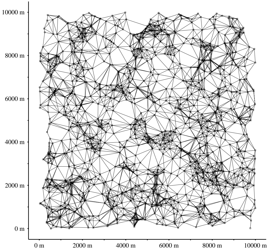
Figure 5.4: Map of the 1,000-station network showing single hops used by routes produced by a modification to minimum-energy routing. Here the cost of a route is a linear combination of the energy and the number of hops. The weightings were ad hoc and chosen to have a moderate effect on the routes.
