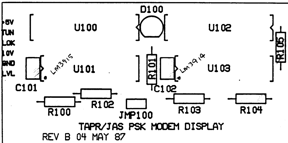
Fig. 1 - Modem Display Parts Placement Guide
