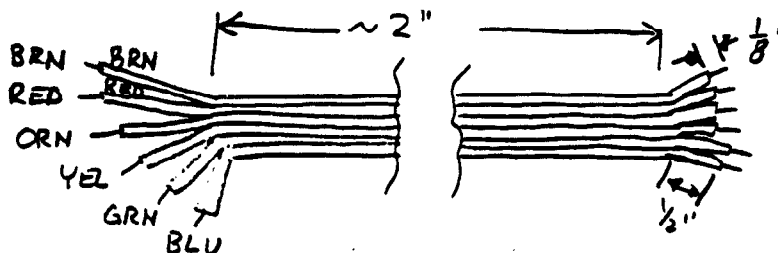
Fig. 3 - 6-Conductor Cable Preparation
