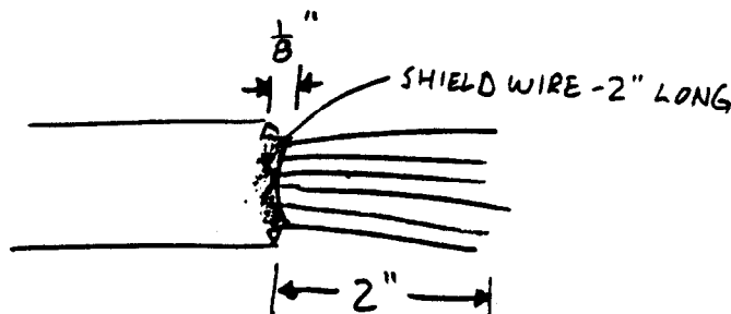
Fig. 9 - Interface Cable Preparation
